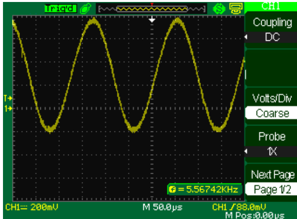
Figure 16 - DC Coupling
