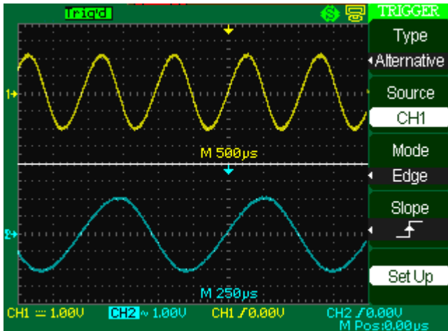
Figure 37 - Alternate Trigger Menu
