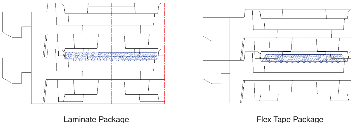
Figure 1: Laminate and Flex Tape BGAs in New Kostat Trays
