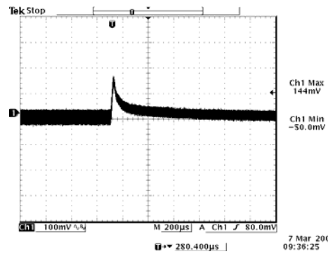
Vout=12 V 100% to 50% Load Transients
