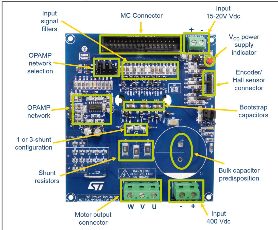
Figure 8: STEVAL-IPMNG8Q architecture
