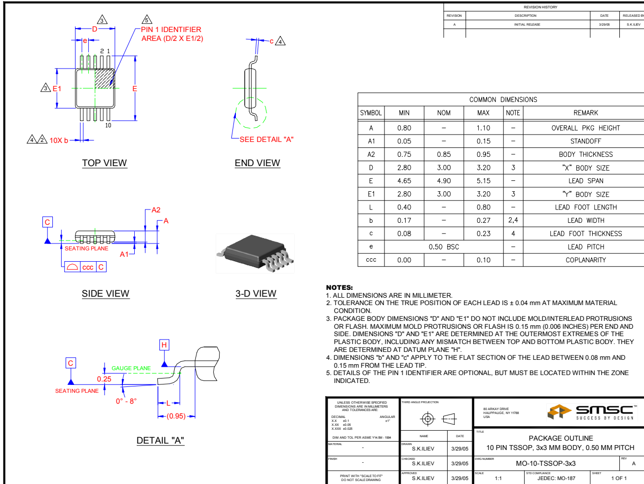
Figure 1 10-Pin MSOP / TSSOP Package
