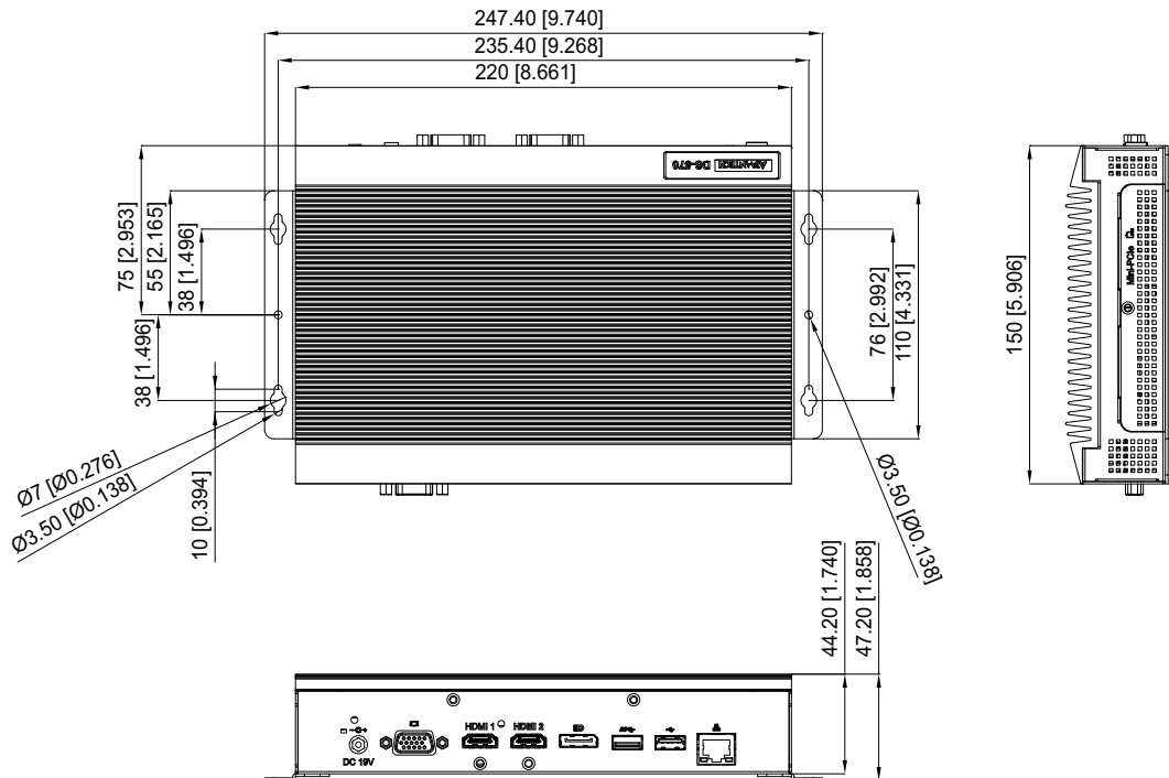
Figure 1.1 DS-570 mechanical dimensions
