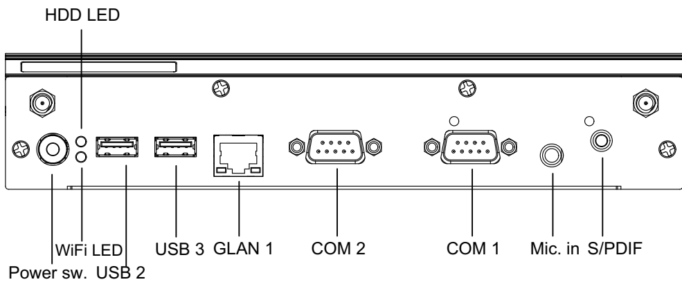
Figure 2.1 Front view
