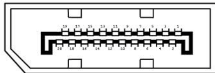
Figure 2.12 DP++ connector
