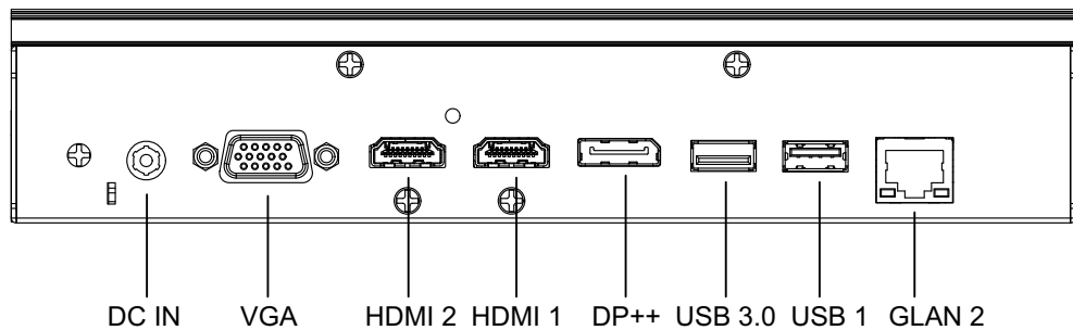
Figure 2.2 Rear view
