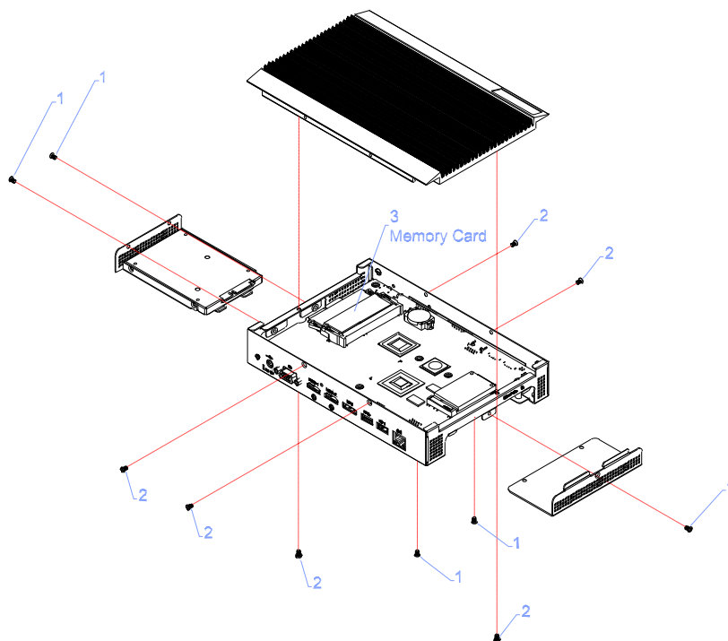
Figure 2.14 Memory module installation
