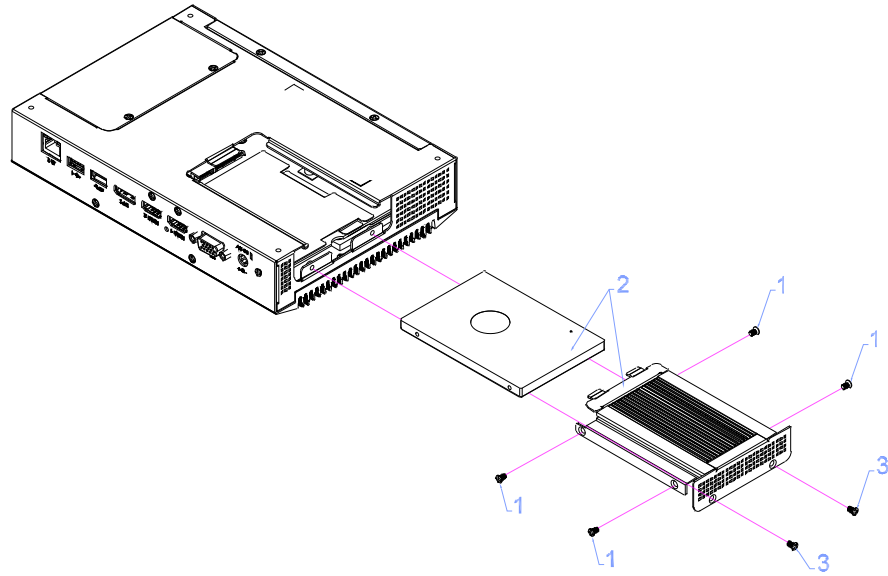
Figure 2.15 HDD installation
