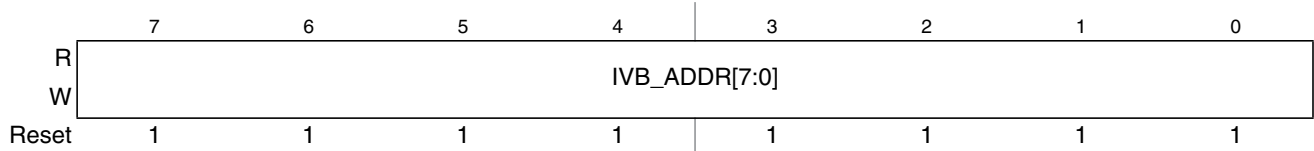
Figure 6-2. Interrupt Vector Base Register (IVBR)
