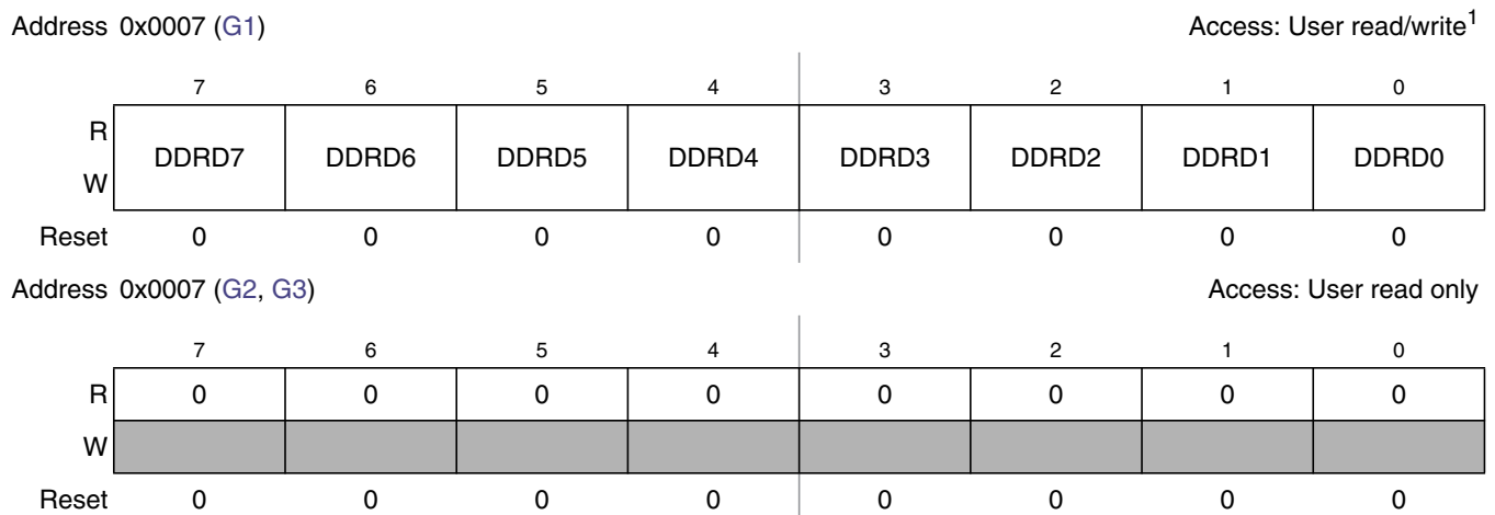
Figure 2-9. Port D Data Direction Register (DDRD)
