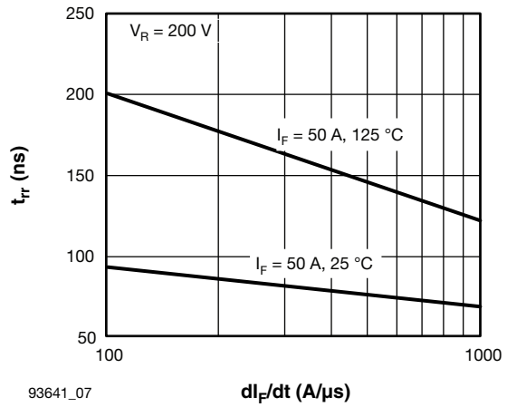
93641_07 di_F/dt (A/μs) Fig. 7 - Typical Reverse/dt Recovery Time vs. di_F/dt
