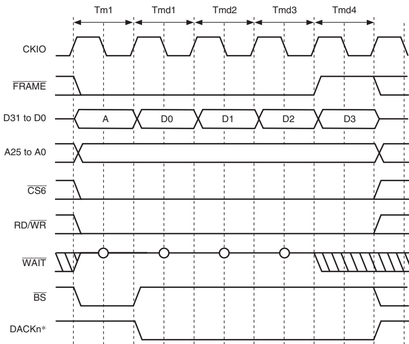
Figure 8.52 Burst MPX Space Access Timing (Burst Write, No Wait, CS6WCR.MPXMD = 0)
