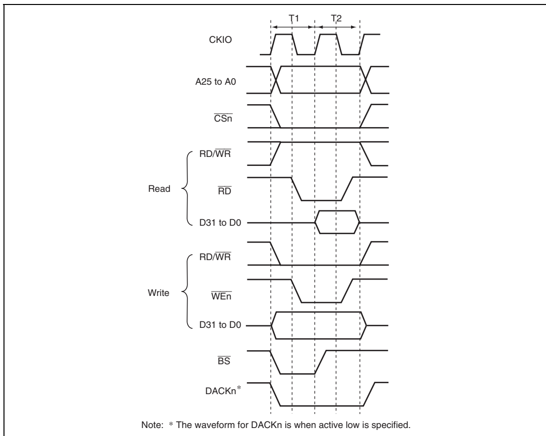
Figure 8.3 Normal Space Basic Access Timing (Access Wait 0)
