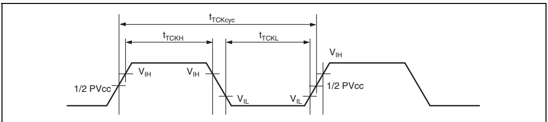
Figure 25.56 TCK Input Timing
