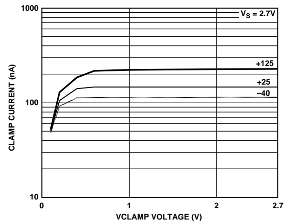
Figure 15. VCLAMP Current Over Temperature at VS = 2.7 vs. VCLAMP Voltage
