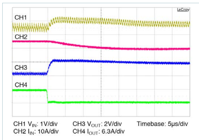
Figure 15 — 6.25A – 0A transient response: C_{IN} = 330\mu\text{F} , I_{IN} measured prior to C_{IN} , no external C_{OUT}
