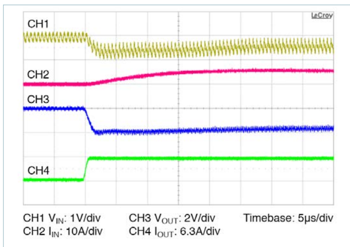
Figure 14 — 0A – 6.25A transient response: C_{IN} = 330\mu\text{F} , I_{IN} measured prior to C_{IN} , no external C_{OUT}
