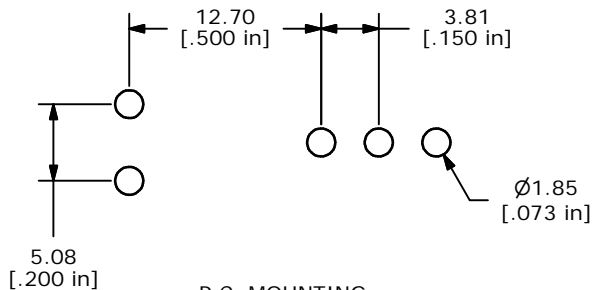
P.C. MOUNTING
