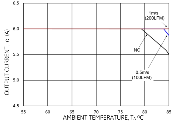
Figure 8. Derating Output Current Temperature versus Ambient Temperature and Airflow.
