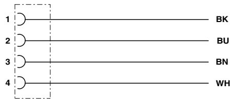
Contact assignment of 7/8" plugs/sockets, cable type 400
