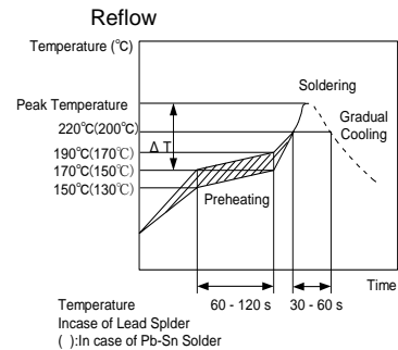
[Standard Conditions for Reflow Soldering]
