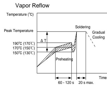
[Allowable Soldering Temperature and Time]
