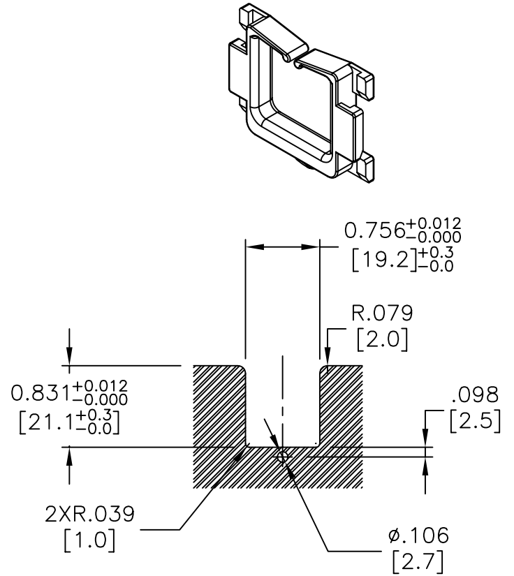
PANEL CUT-OUT DETAIL
