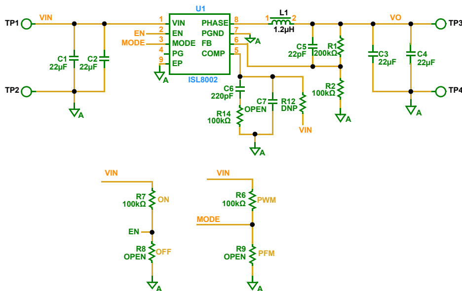
FIGURE 1. ISL8002DEMO1Z SCHEMATIC
