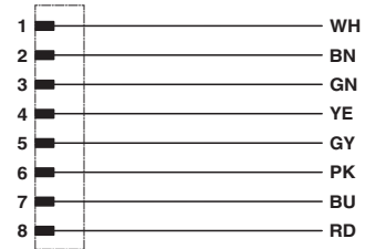
Contact assignment of the M12 plug
