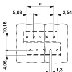
Drilling diagram
