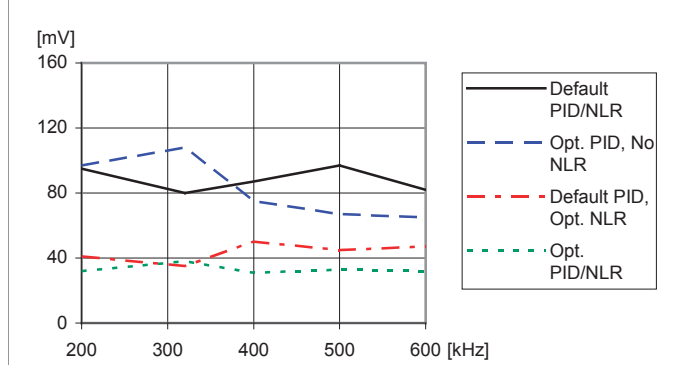
Load transient peak voltage deviation vs. frequency. Step-change (5-15-5 A). T_{P1} = +25 °C, V_I = 12 V, V_O = 1.0 V, C_O = 470 \mu F/10 m \Omega
