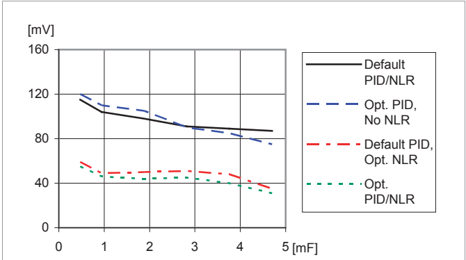
Load transient peak voltage deviation vs. external capacitance. Step-change (5-15-5 A). Parallel coupling of capacitors with 470 \mu F/10 m \Omega , T_{P1} = +25 °C, V_I = 12 V, V_O = 3.3 V, f_{sw} = 320 kHz, di/dt = 2 A/ \mu s
