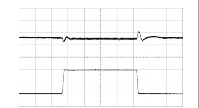
Output voltage response to load current step-change (5-15-5 A) at: T_{P1} = +25 °C, V_I = 12 V, V_O = 1.0 V, di/dt = 2 A/ \mu s, f_{sw} = 320 kHz, C_O = 470 \mu F/10 m \Omega Top trace: output voltage (200 mV/div.). Bottom trace: load current (5 A/div.). Time scale: (0.1 ms/div.).
