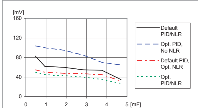
Load transient peak voltage deviation vs. external capacitance. Step-change (5-15-5 A). Parallel coupling of capacitors with 470 \mu F/10 m \Omega , T_{P1} = +25 °C, V_I = 12 V, V_O = 1.0 V, f_{sw} = 320 kHz, di/dt = 2 A/ \mu s
