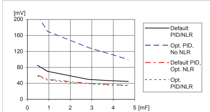
Load Transient vs. External Capacitance, V_O = 1.0 V
