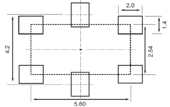
Figure 2) Land Pattern
