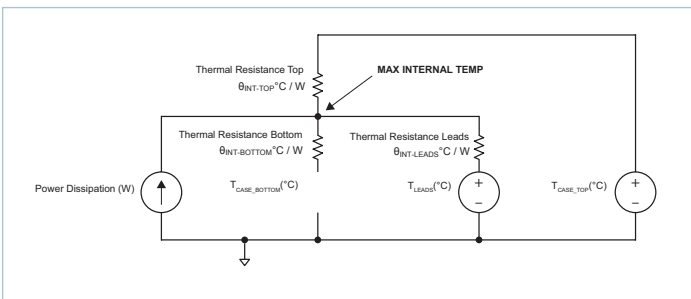
Figure 23 — One-side cooling and leads thermal model
