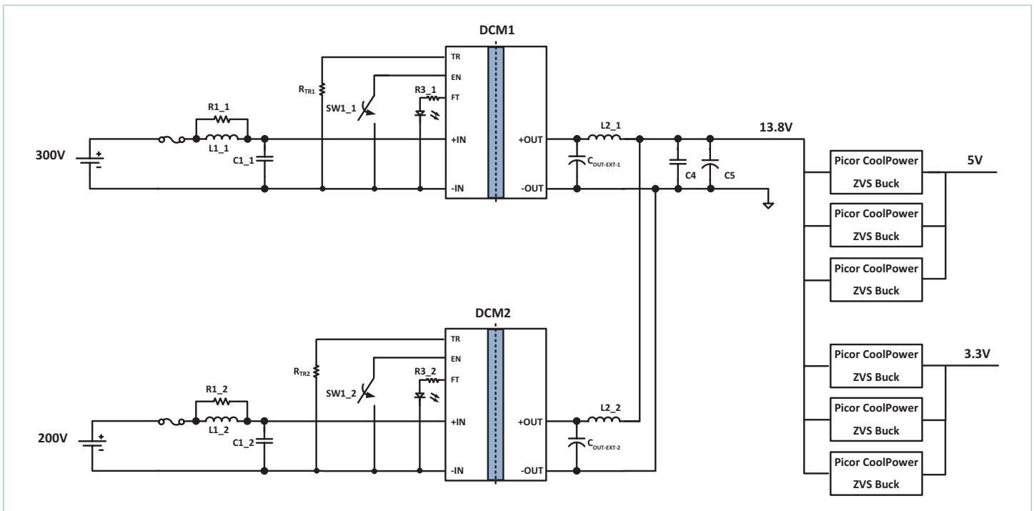
Typical Application 2: DCM4623xC8G16F0yzz + Picor Point-of-Load
