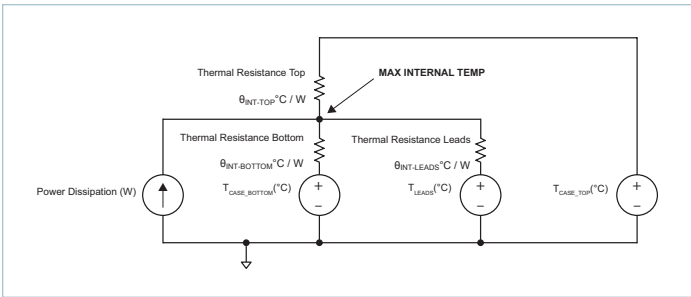
Figure 22 — Double-side cooling and leads thermal model
