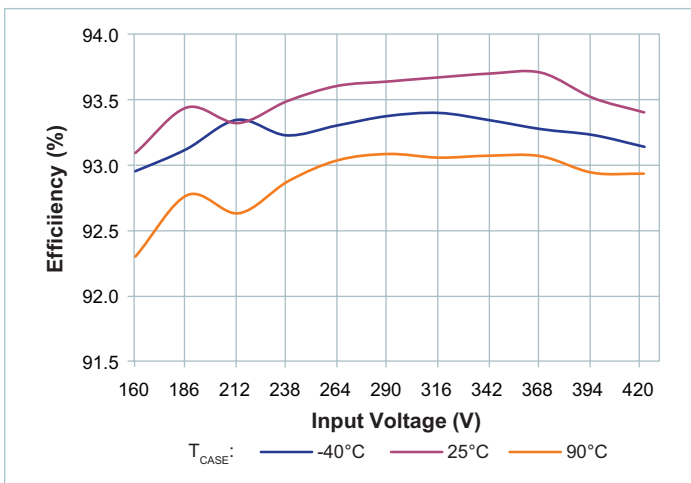
Figure 9 — Full load efficiency vs. V_{IN} , V_{OUT} = 15.5V
