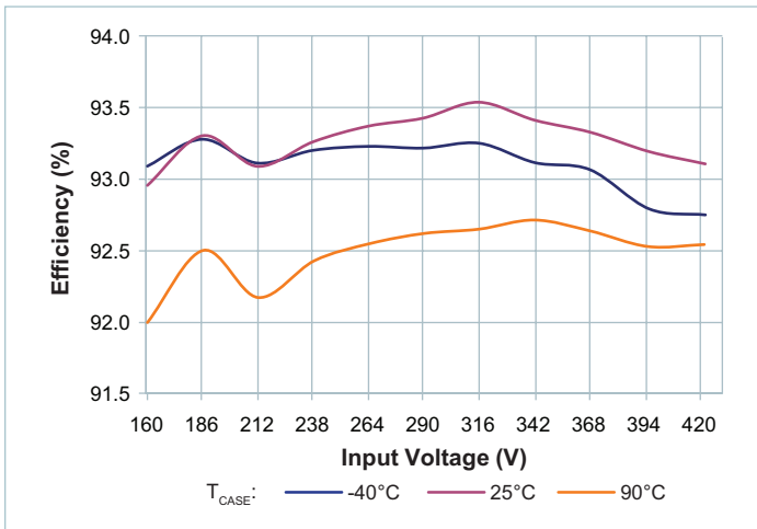
Figure 7 — Full load efficiency vs. V_{IN} , V_{OUT} = 11.5V
