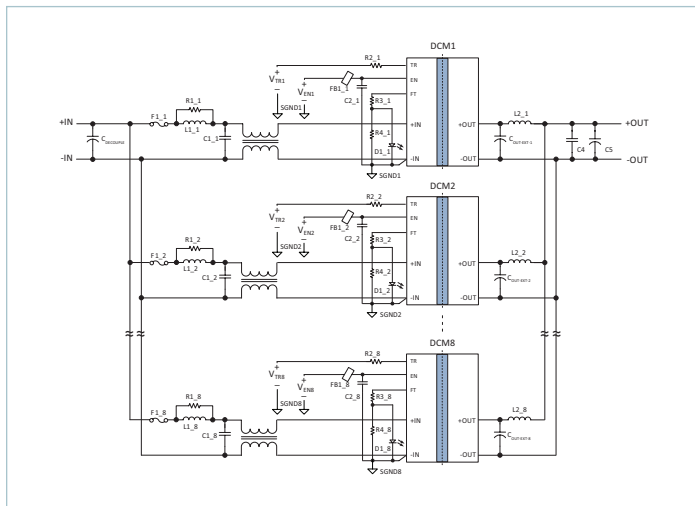
Figure 26 — DCM paralleling configuration circuit 2
