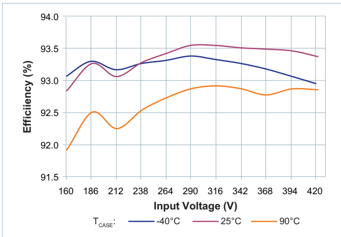
Figure 8 — Full load efficiency vs. V_{IN} , V_{OUT} = 13.8V
