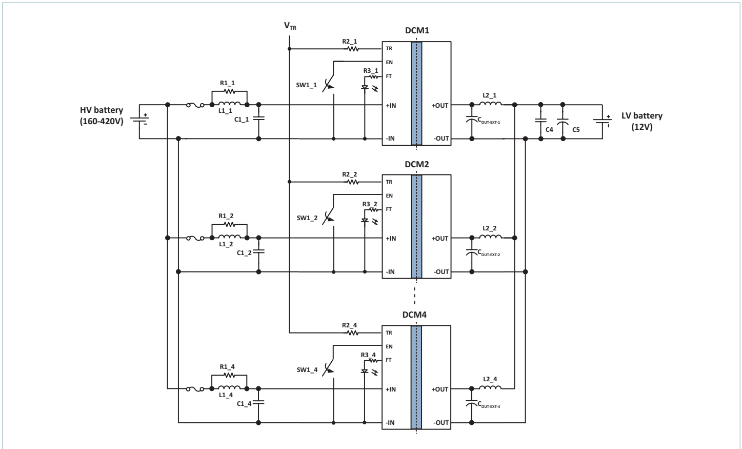
Typical Application 1: DCM4623xC8G16F0yzz for EV/HEV applications
