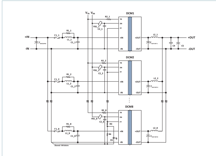
Figure 25 — DCM paralleling configuration circuit 1
