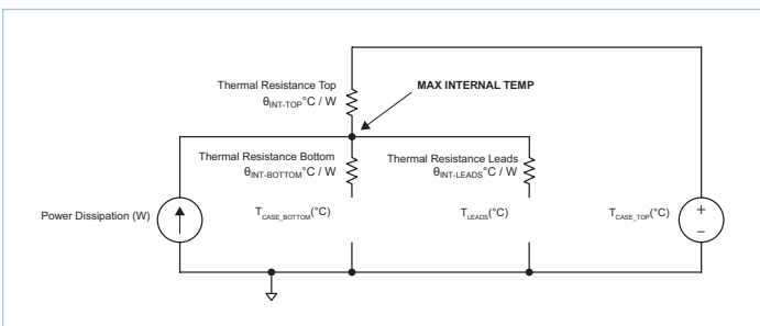
Figure 24 — One-side cooling thermal model
