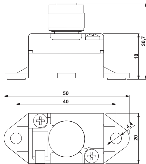
Dimensioned drawing
