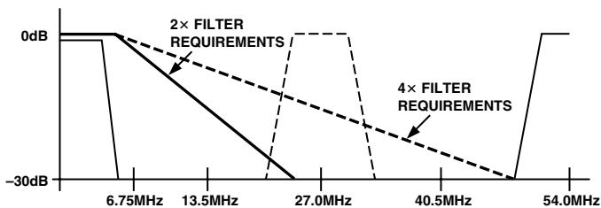
Figure 35b. Output Filter Requirements in 4x Oversampling Mode
