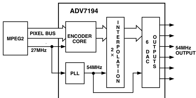
Figure 35a. PLL and 4x Oversampling Block Diagram
