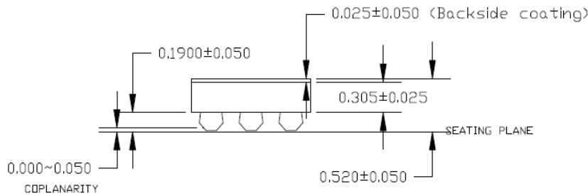
SIDE VIEW NOTE: 1, 2
