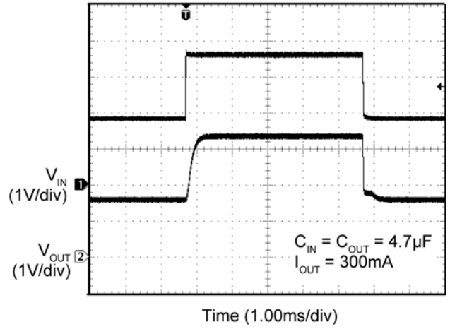
Line Transient
