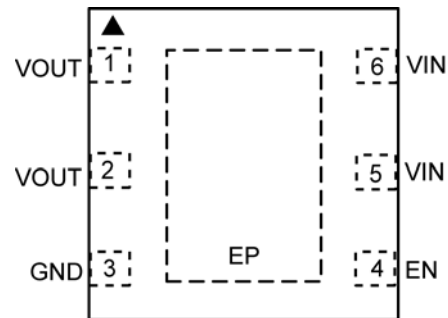
6-Pin 1.6mm × 1.6mm Thin DFN (MT) Top View
