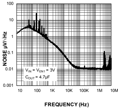
MIC94305YMT Output Noise Spectral Density
