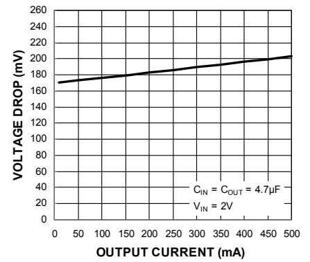
Voltage Drop vs. Output Current
