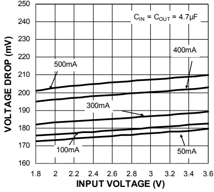
Voltage Drop vs. Input Voltage
