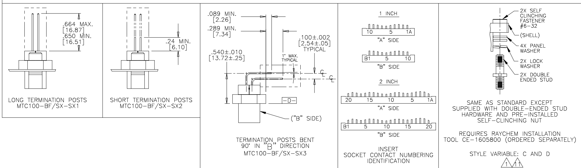
FIGURE 1 BASIC DESIGN VARIATIONS
