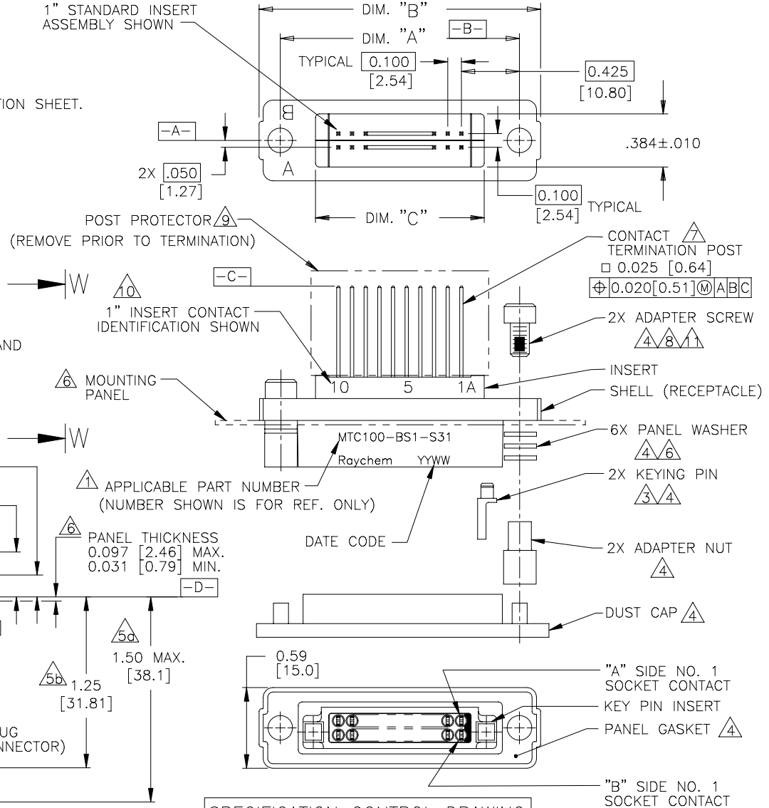
SPECIFICATION CONTROL DRAWING
