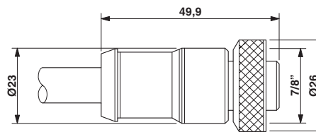
Dimensioned drawing
