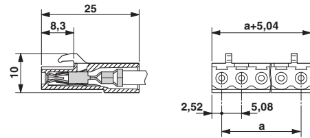
Dimensioned drawing
