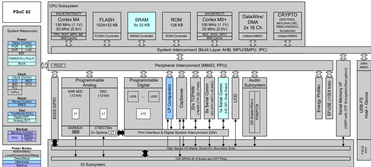
Figure 2. Block Diagram
