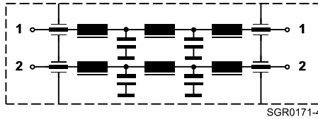
Circuit diagram 1
