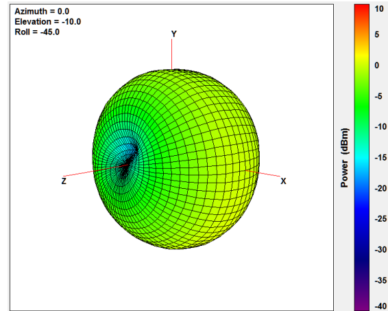
824MHz
