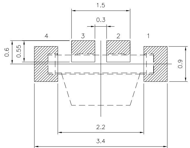
Recommend Soldering pad
