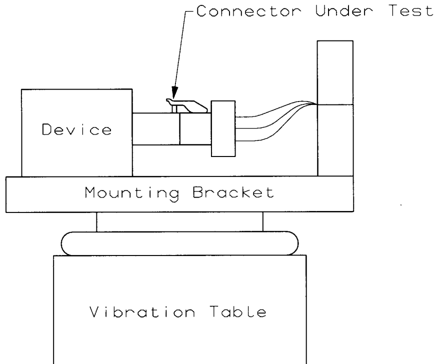
Figure 5 Vibration & Mechanical Shock Mounting Fixture
