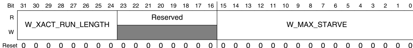
DDRC_PERFWR1 field descriptions
