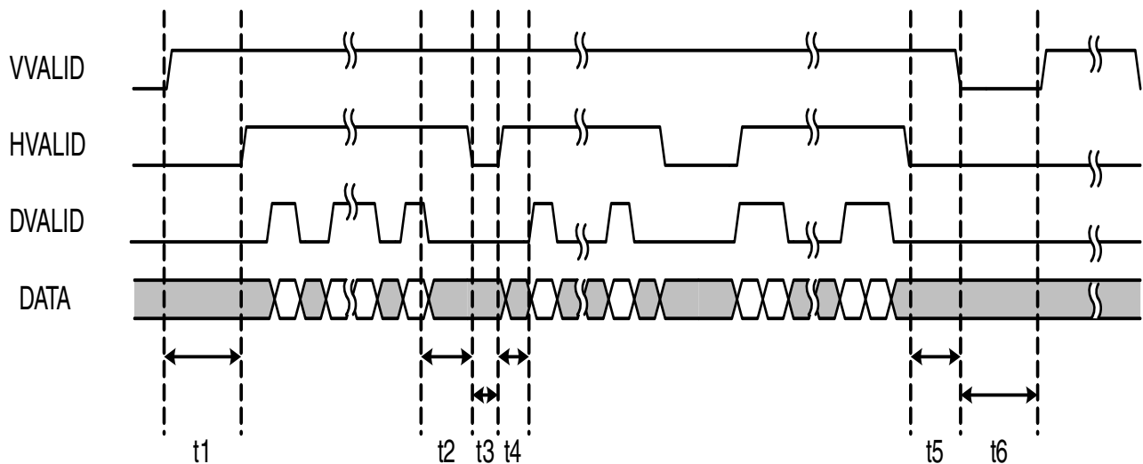
Figure 13-55. Timing Diagram of ISP Wrapper Output Protocol
