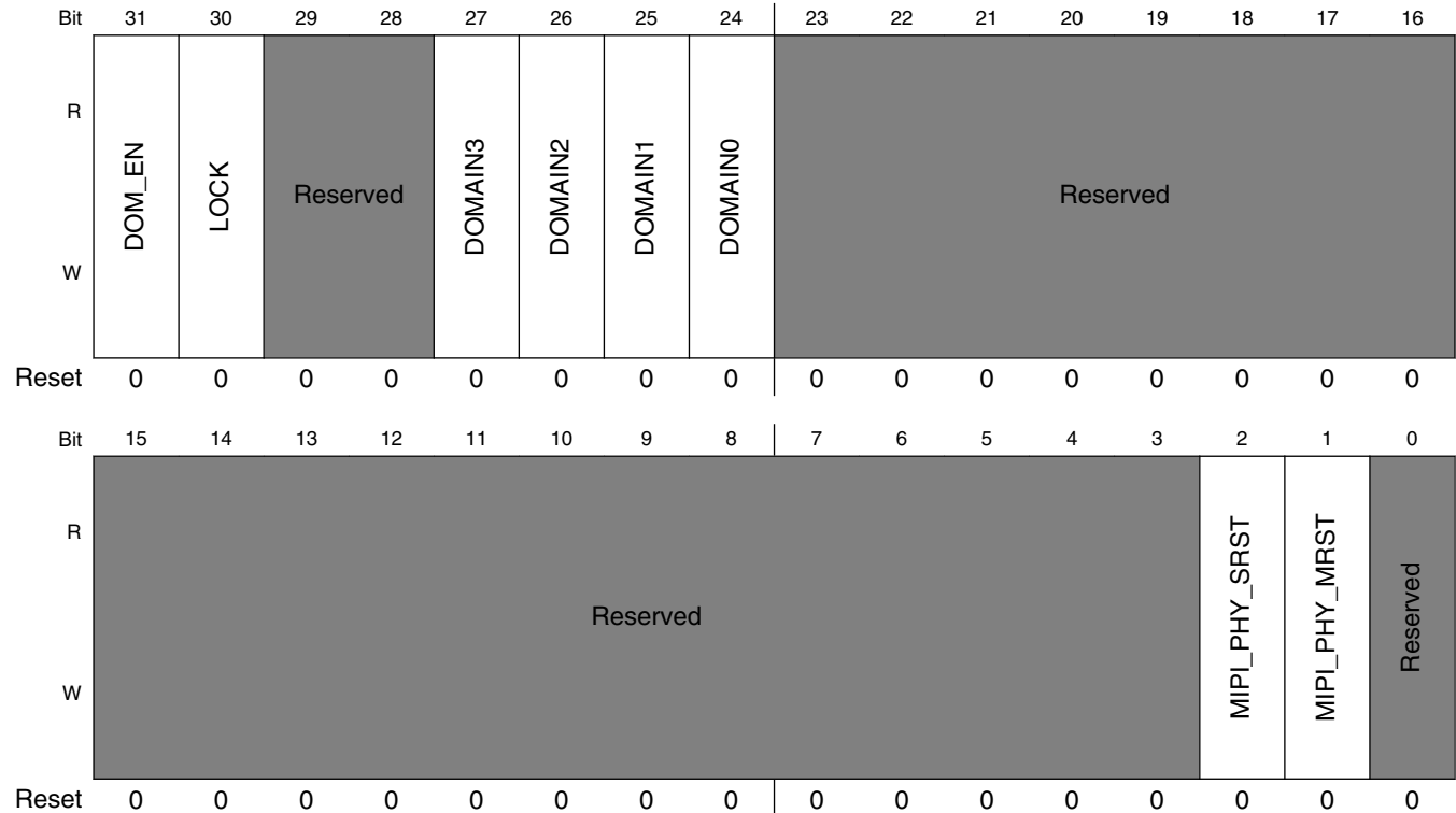
SRC_MIPIPHY_RCR field descriptions
