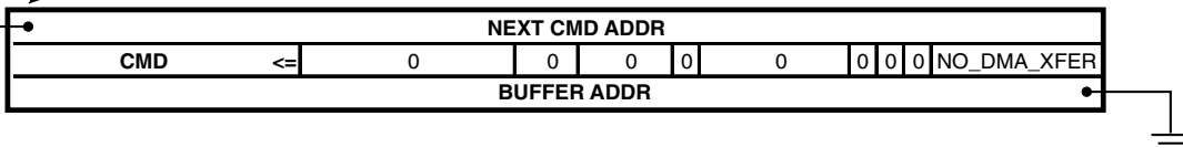
Figure 9-37. BCH Decode DMA Descriptor Chain
