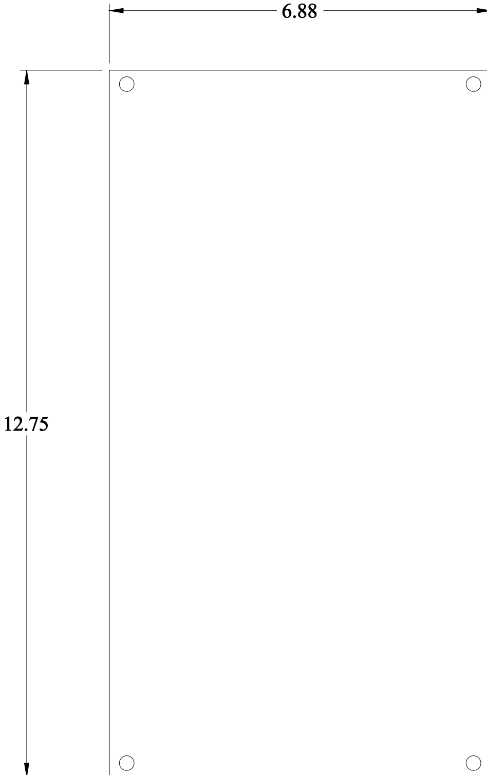
FRONT VIEW
